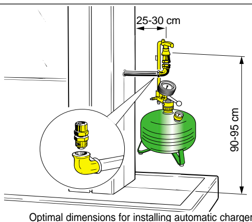
Optimal dimensions for installing automatic charger
